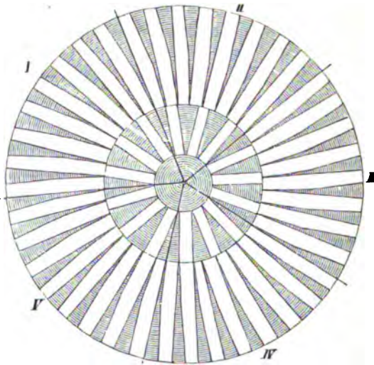
Fig. 341.—Staves shown in a cross-section of oak.
